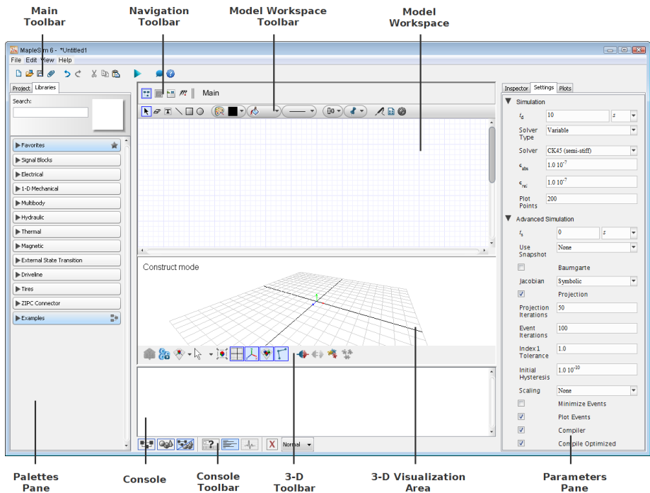
Figure 1.7: MapleSim Window
