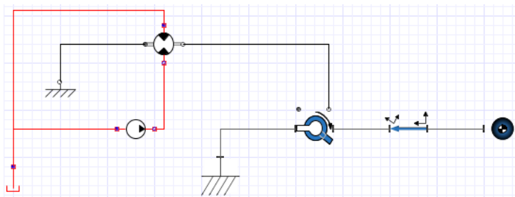
Figure 6.20: Rotational Fixed Flange Hydraulic component
