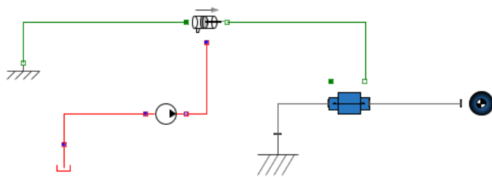
Figure 6.19: Translational Fixed Flange Hydraulic component
