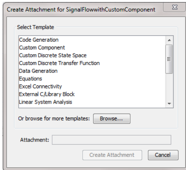
Figure 3.1: MapleSim Templates
