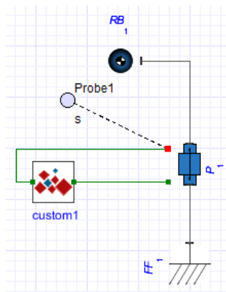
Figure 6.7: Bouncing Ball
