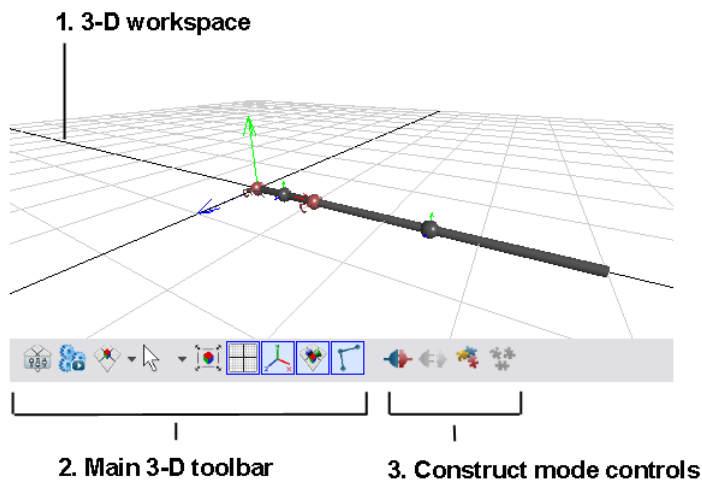
Figure 4.5: 3-D Workspace
