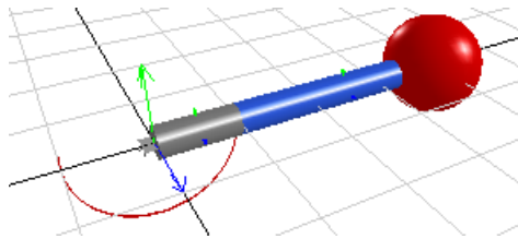
Figure 4.10: Attached Shapes
