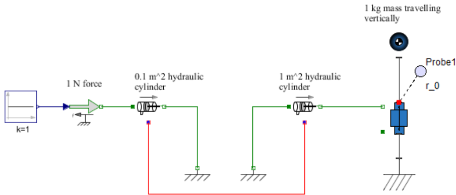
Figure 6.21: Pascal's Principle Example
